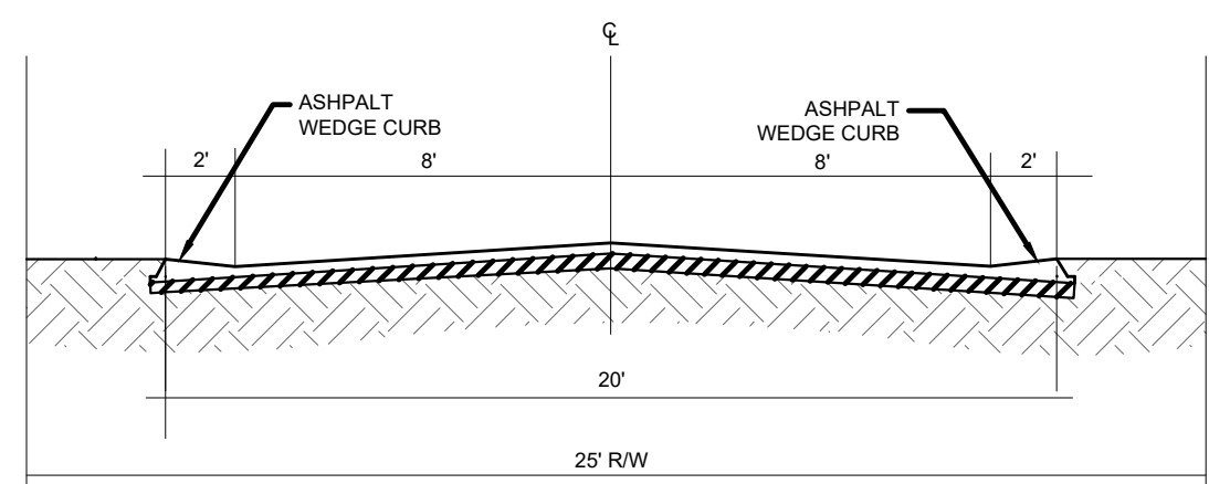
25' RIGHT-OF-WAY (RESIDENTIAL PRIVATE ALLEY) SECTION
