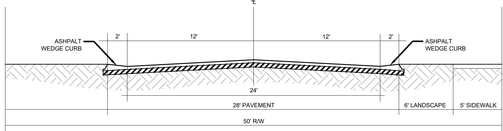
50' RIGHT-OF-WAY (RESIDENTIAL STREET) SECTION (PER CONCEPTUAL DEVELOPMENT PLAN)
